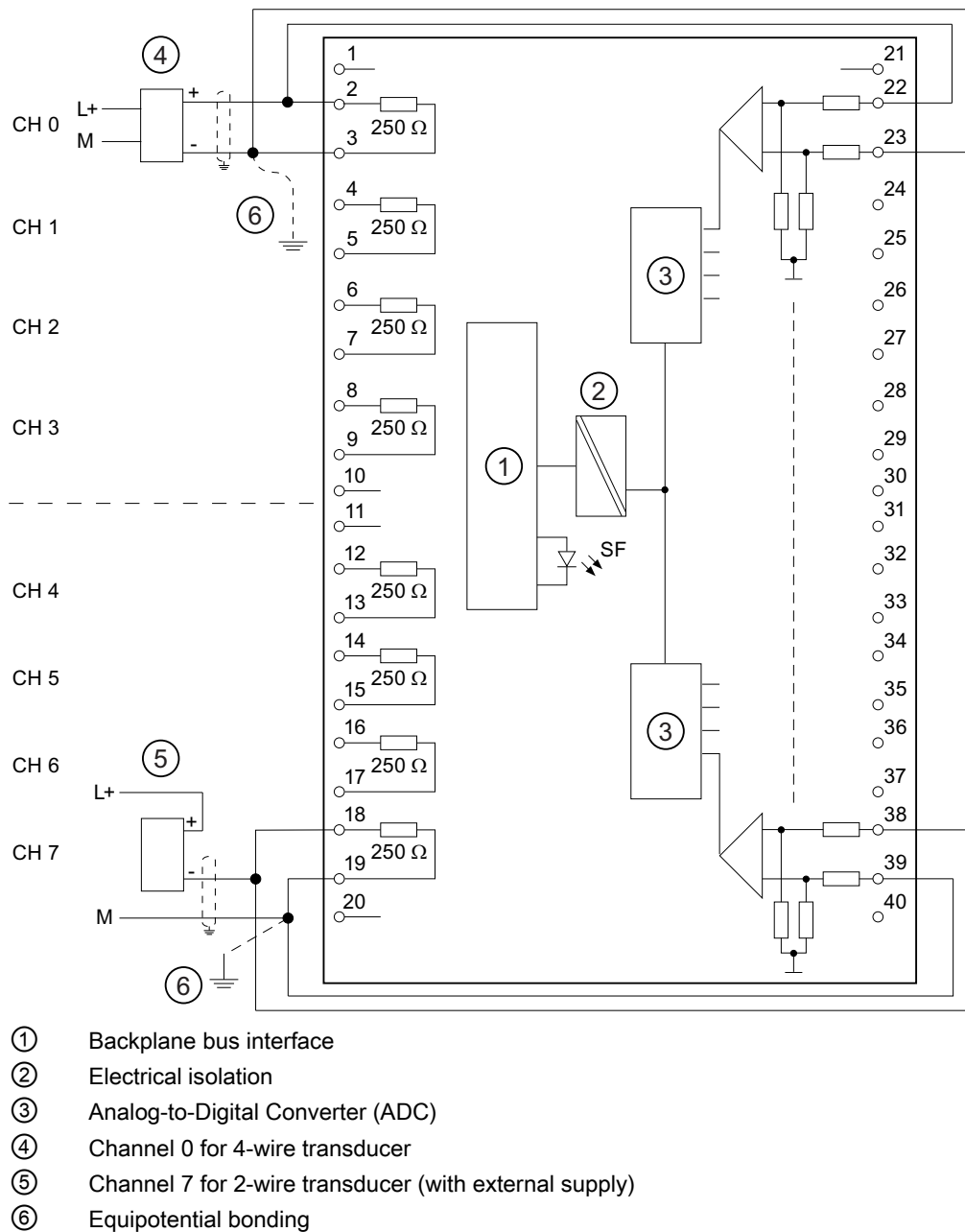
Figure 6-2 Wiring and block diagrams
