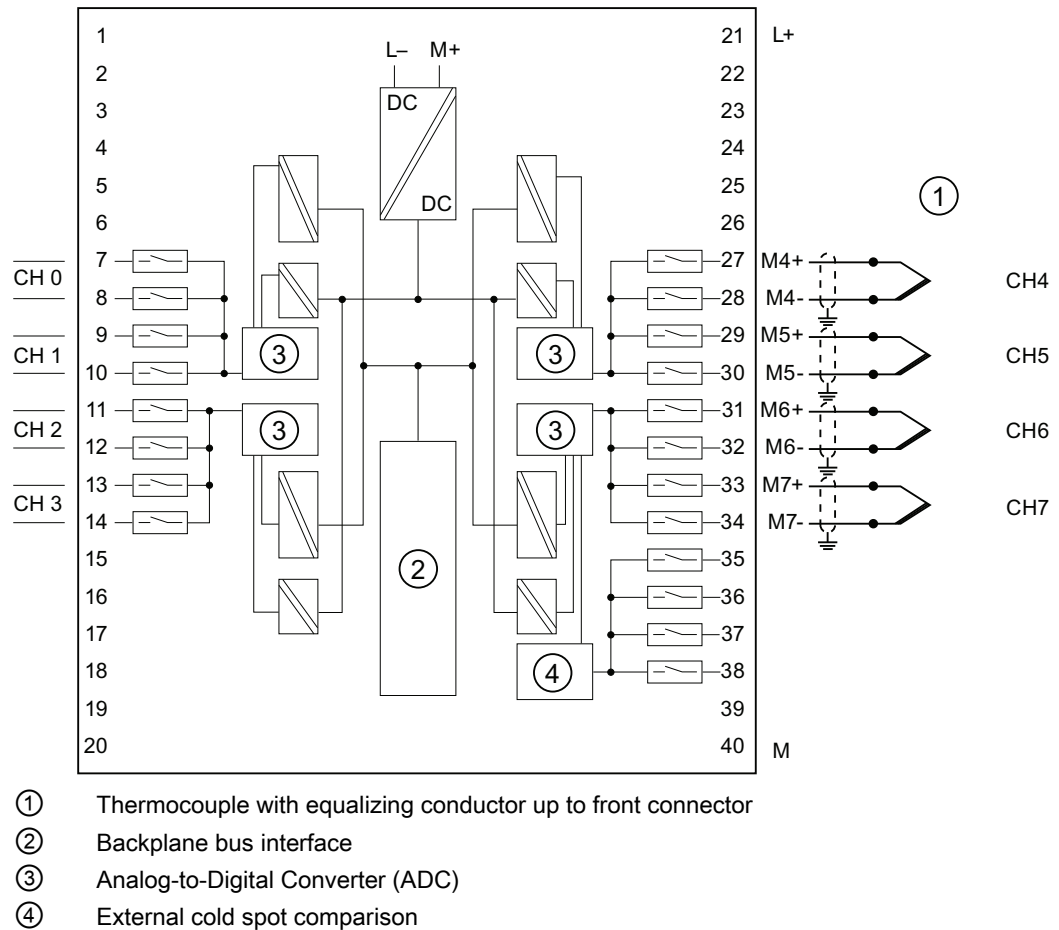
Figure 6-28 Wiring and block diagrams
