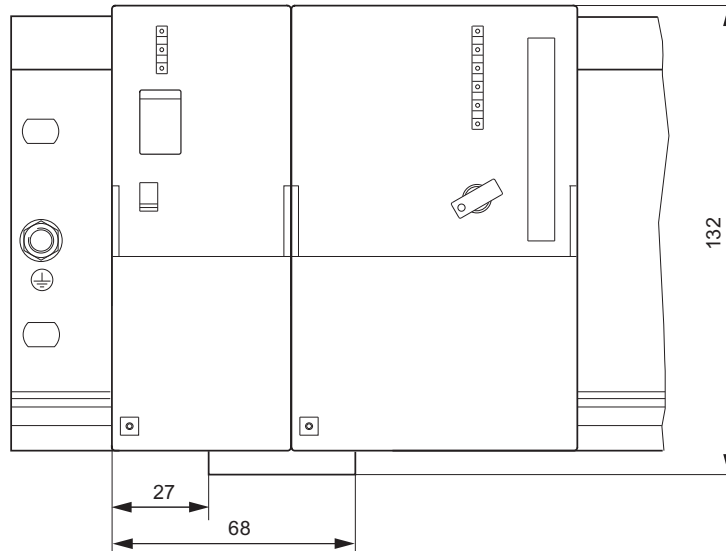
Figure C-12 Dimensional drawing of power supply module PS 307; 10 A with CPU 313/314/315/315-2 DP, front view
