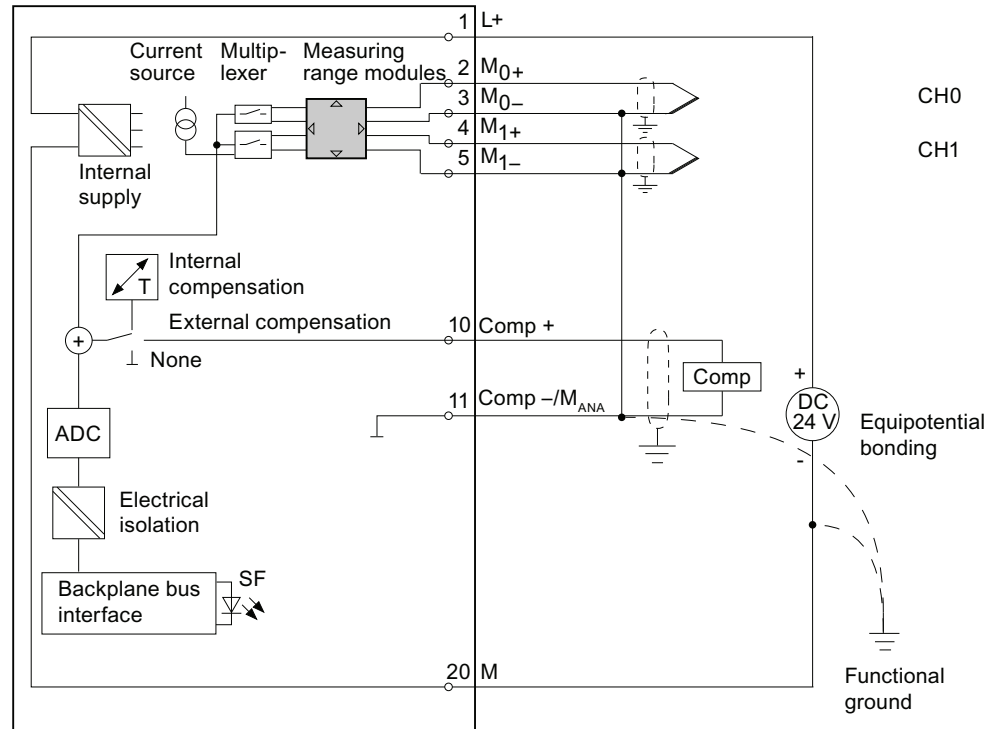
Figure 6-18 Wiring and block diagrams
