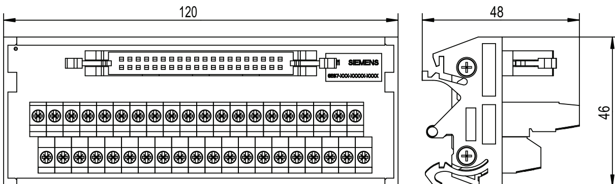
Figure C-21 40-pin terminal block
