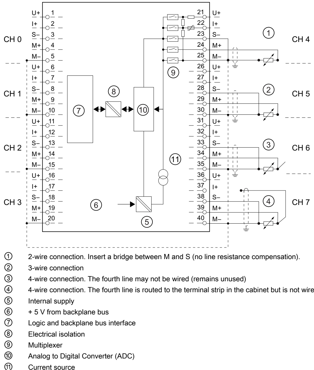
Figure 6-12 Block diagram and terminal diagram
