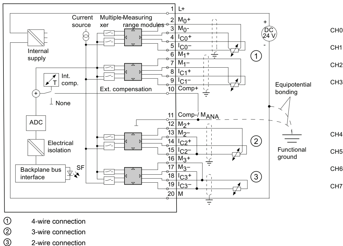
Figure 6-15 Block diagram and terminal diagram
