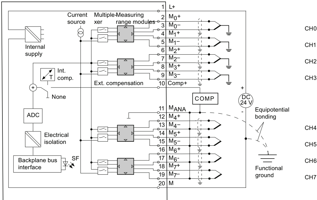
Figure 6-16 Block diagram and wiring diagram
