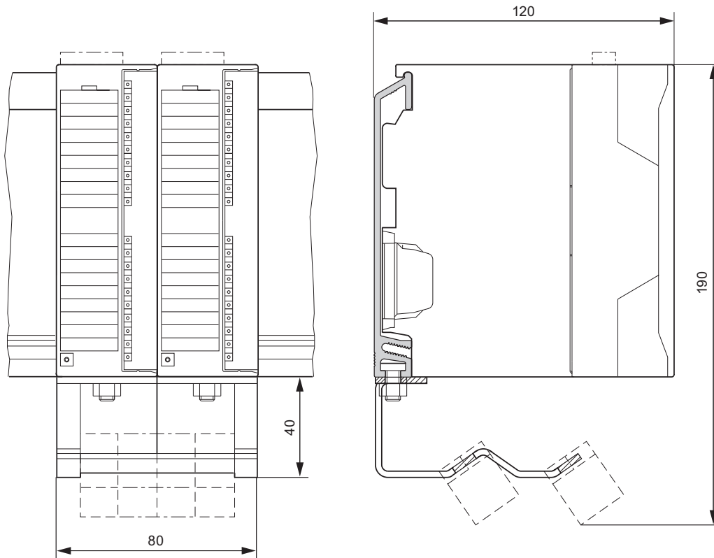
Figure C-20 2 signal modules with shield connecting element
