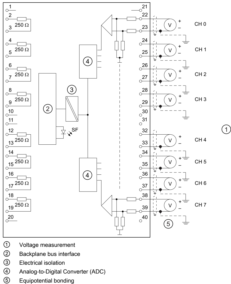
Figure 6-1 Wiring and block diagrams
