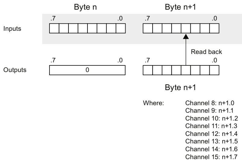
Figure 3-9 Readback of the outputs of SM 327; DI 8/DO 8 x DC 24 V/0.5 A
