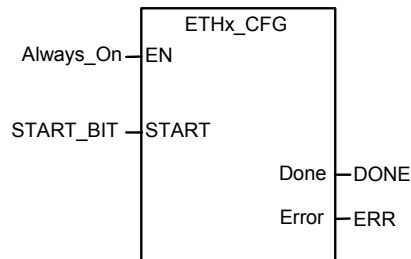
Fig. 10 Call of the subprogram ETHx_CFG
