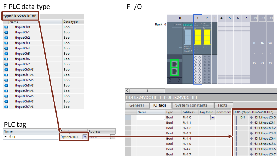
Figure 5-6: Access to I/O areas with F-PLC data types
