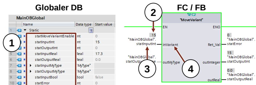
Figure 2-2: Terms for tags and parameters
