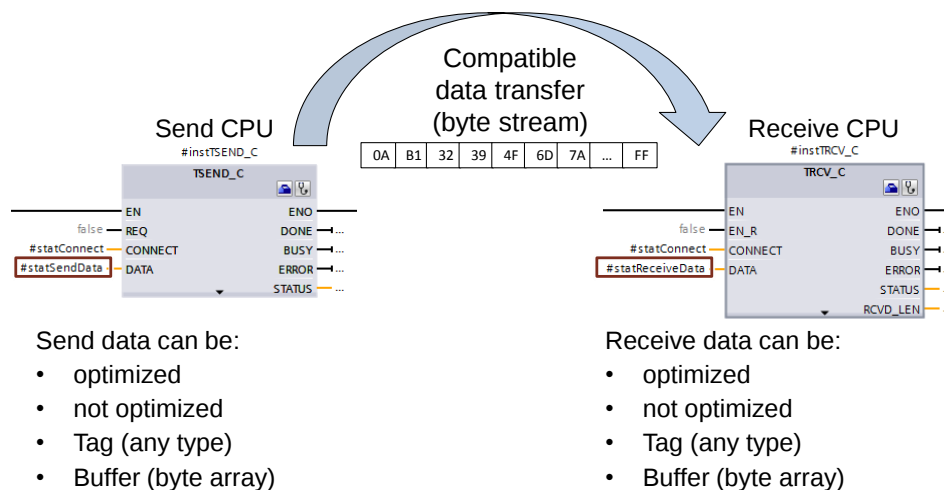
Figure 2-11: CPU-CPU communication
